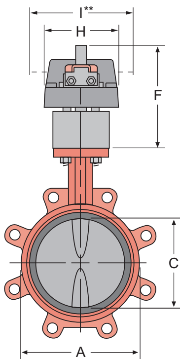
FRONT VIEW
